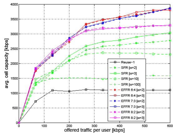
Fig. 7. Mean uplink cell capacity of three frequency reuse schemes with different power ratios as a function of offered traffic per user, 25 users are uniformly distributed in each cell in the system.
