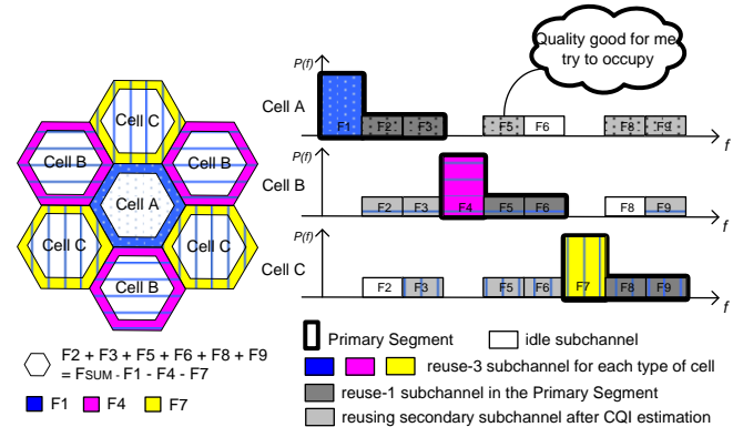
Fig. 2. Concept of the EFFR scheme in a cellular system based on partition of exclusively reuse-3 subchannels and reuse-1 subchannels in the Primary Segment, as well as interference-aware reuse on the Secondary Segment.
