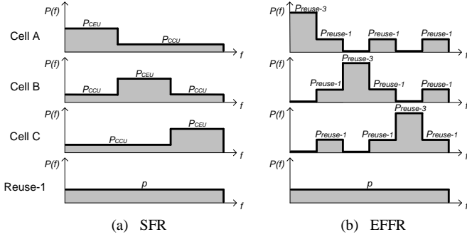
Fig. 3. Cell-specific power masks over system bandwidth for the SFR scheme and the EFFR scheme.
