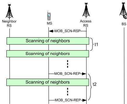
Figure 4. Scanning and reporting periods when no data are transmitted (de-centrally controlled RS)
