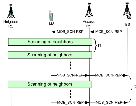
Figure 5. Scanning and reporting periods when no data are transmitted (centrally controlled RS)
