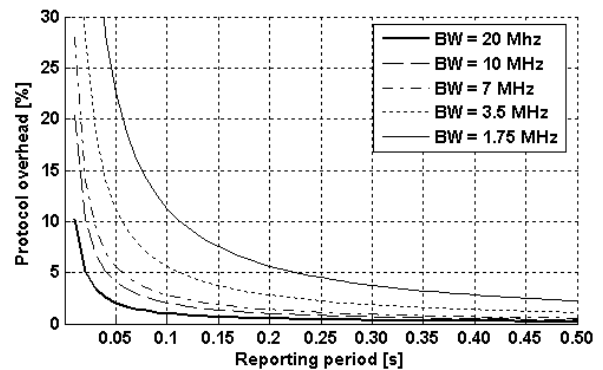
Figure 9. Protocol overhead in dependence on system bandwidth and reporting period (50 active users is considered)
