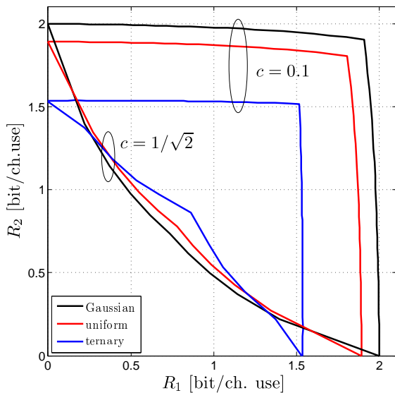
Fig. 1. Achievable rate regions of Gaussian-, uniformly-, and ternary-distributed codes: fully symmetric GIC with P = 15 and c = \{0.1, 1/\sqrt{2}\} .
