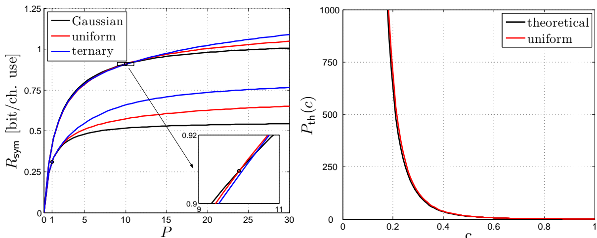
Fig. 2. Achievable symmetric rate of Gaussian-, uniformly-, and ternary-distributed codes for two different values of c yielding theoretical threshold powers of 1 and 10 (left). Comparison between the theoretical value of the threshold and the actual value of achieved by uniformly-distributed codes (right).
