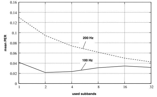
Fig. 7. Mean PER with arrival rate of one MPDU per MAC frame
