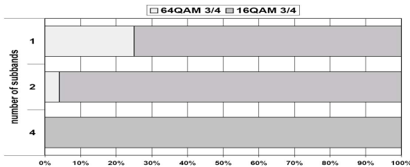
Fig. 9. PHY mode usage at system saturation (100% resource utilization)
