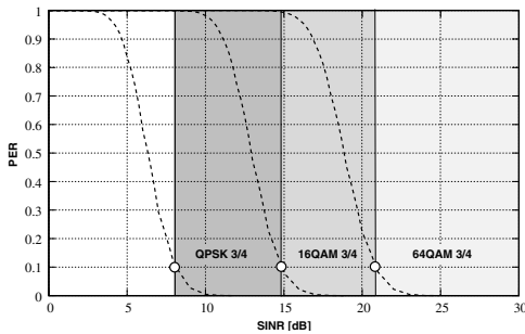
Fig. 3. PER curves and PHY mode ranges
