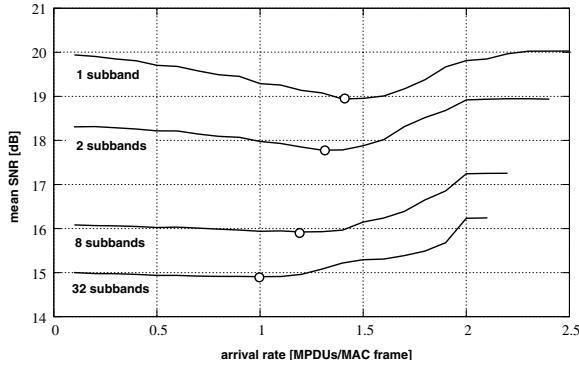
Fig. 5. Mean SNR with 100 Hz Doppler shift
