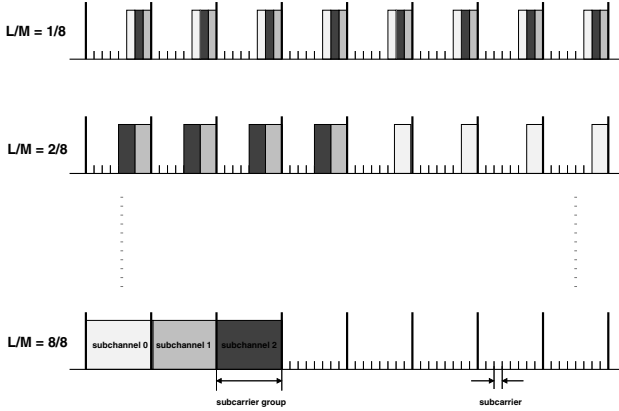
Fig. 1. Mapping of logical subchannels onto physical resources in the frequency domain ( M : subcarriers per subchannel, L : subcarriers from the same subband in a subchannel)
