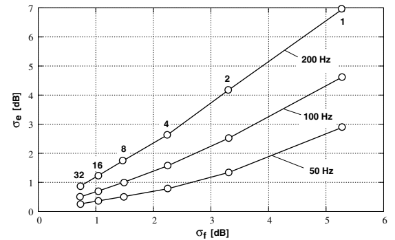
Fig. 4. Dependency between standard deviation of fading level ( \sigma_f ) and estimation error ( \sigma_e ) for different OFDMA subchannel mapping schemes (the conditional estimation accuracy depending on the current fading level is not investigated in detail)
