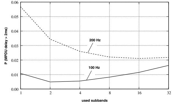
Fig. 8. MPDU delay with arrival rate of one MPDU per MAC frame
