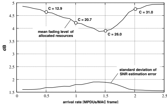
Fig. 6. Standard deviation of SNR estimation error and mean fading level of scheduled resources with 100 Hz Doppler shift for mapping of a subchannel onto a single subband; C is the mean number of data connections with MPDUs in the transmission queue
